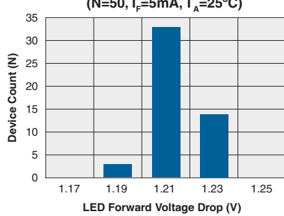
Typical LED Forward Voltage Drop (N=50, I_F=5\text{mA} , T_A=25^\circ\text{C} )
