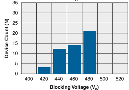
Form-A Typical Blocking Voltage Distribution (N=50, T_A=25^\circ\text{C} )
