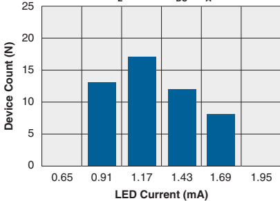
Form-A Typical I_F for Switch Operation (N=50, I_L=120\text{mA}_{DC} , T_A=25^\circ\text{C} )
